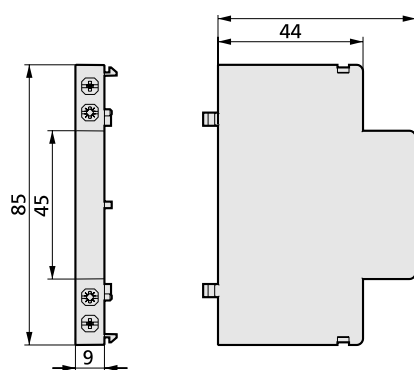
Auxiliary contact
